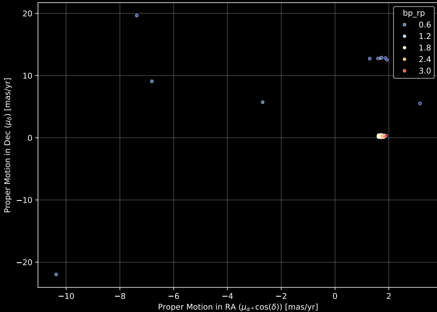
APOGEE DR17 Field: [279-33-O] Proper Motion Diagram (n= 56)
