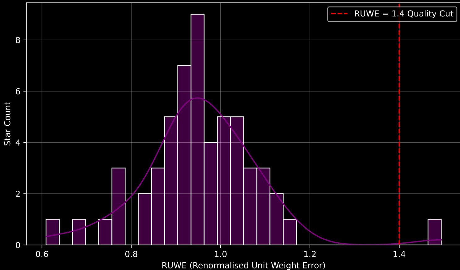
GAPOGEE DR17 Field [279-33-O] RUWE Distribution (n= 56)
