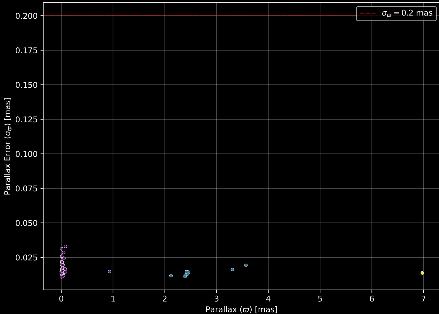
APOGEE DR17 Field: [279-33-O] Parallax Quality (n= 56)
