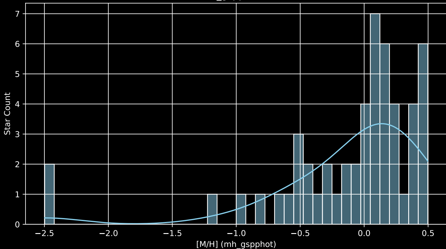
APOGEE DR17 Field: [279-33-O [M/H] (mh_gspphot) (n= 52)
