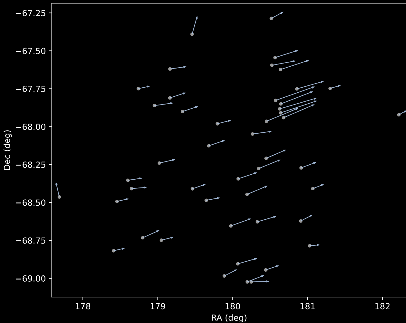
APOGEE DR17 Cluster 1 Proper Motion Vectors (n=47)
