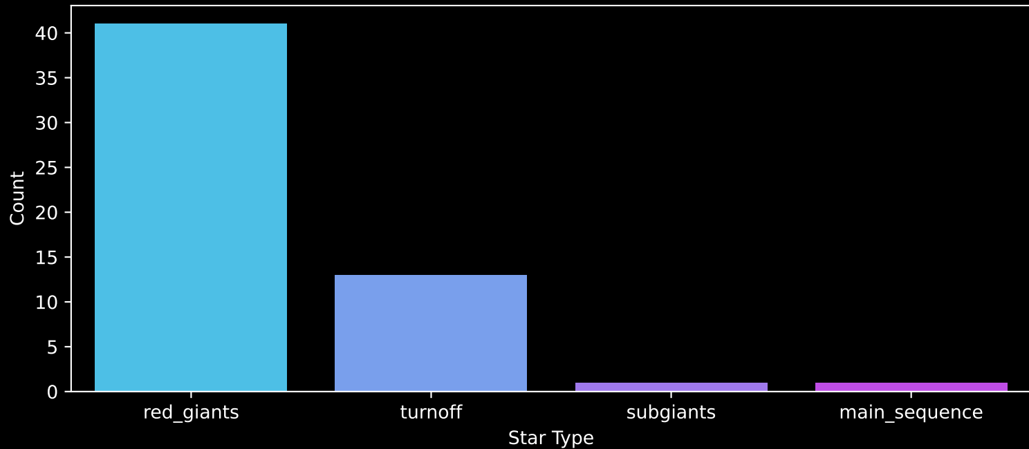
APOGEE DR17 Field: [279-33-O] Count plot of Star Type
