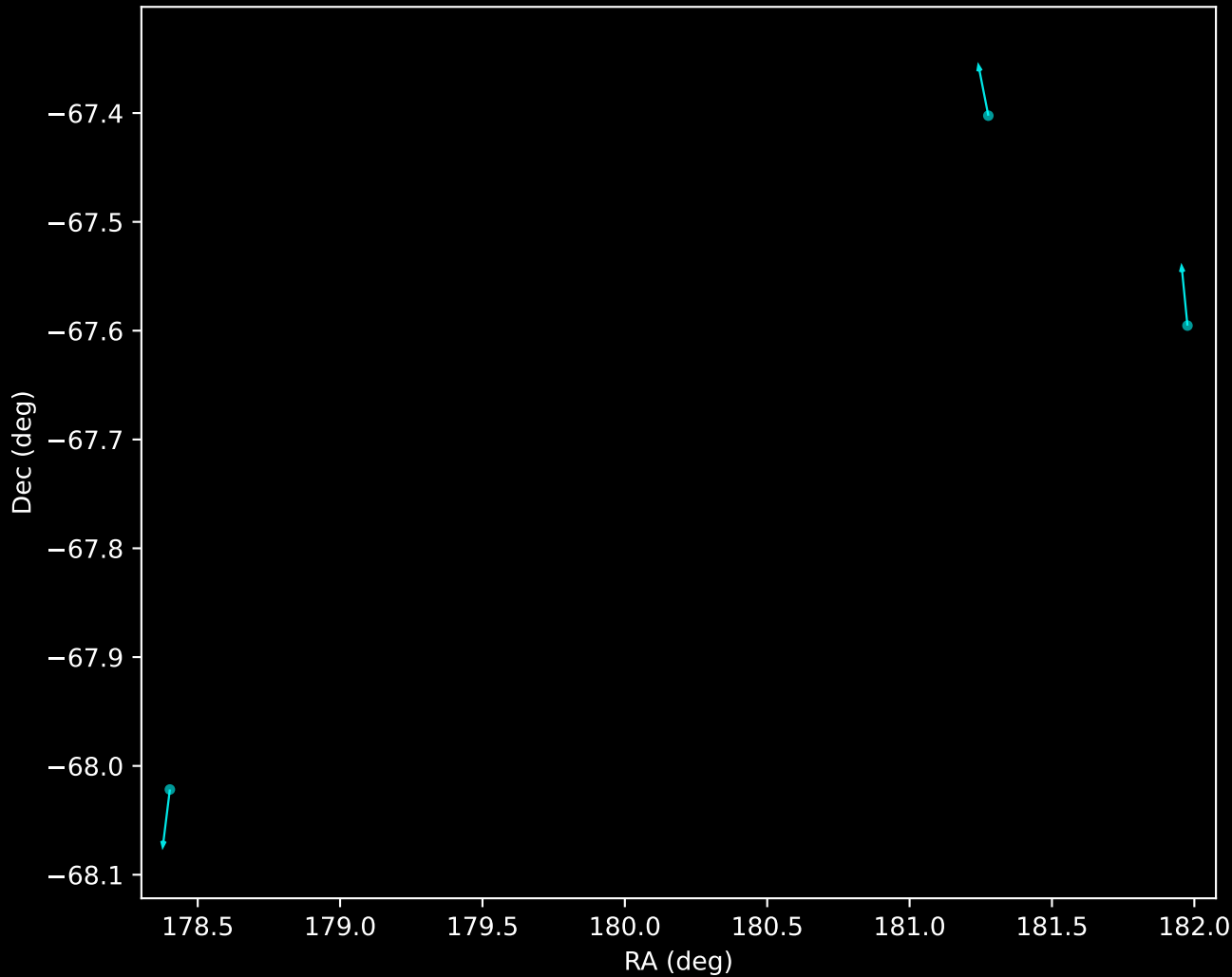
APOGEE DR17 Noise Stream Proper Motion Vectors (n=3)
